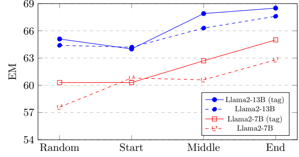
Figure 7: The experimental results of using the “<KEY>” tag to guide LLM on the RAG task at different order of documents. The solid line is the result of adding the “<KEY>” tag, while the dashed line is the baseline result.
