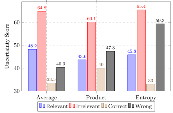
(b) Three different uncertainty estimations.
